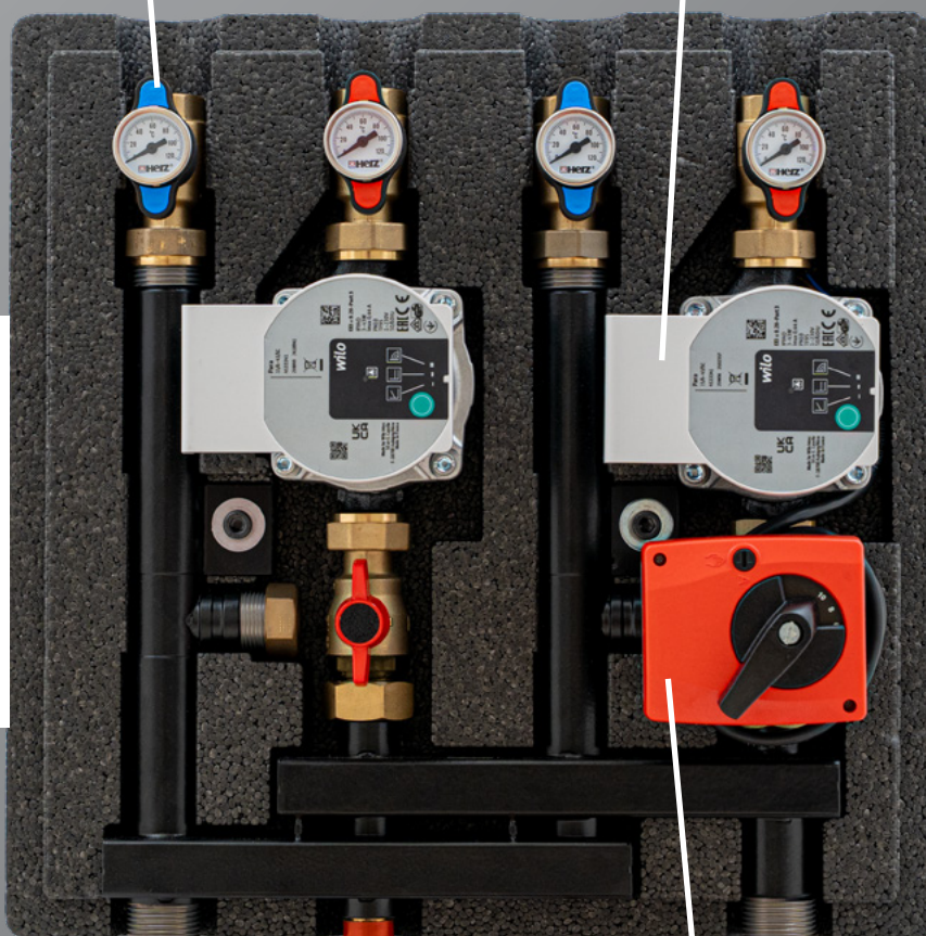
Ball valve with thermometer and check valve
